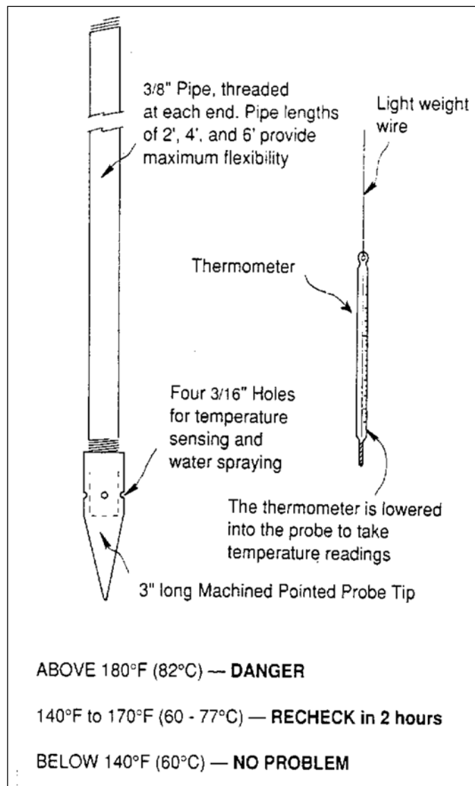
Diagram 9. Temperature Probe
